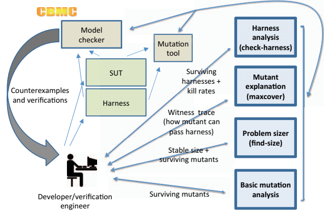
Fig. 6. Basic flow of falsification-driven verification.
