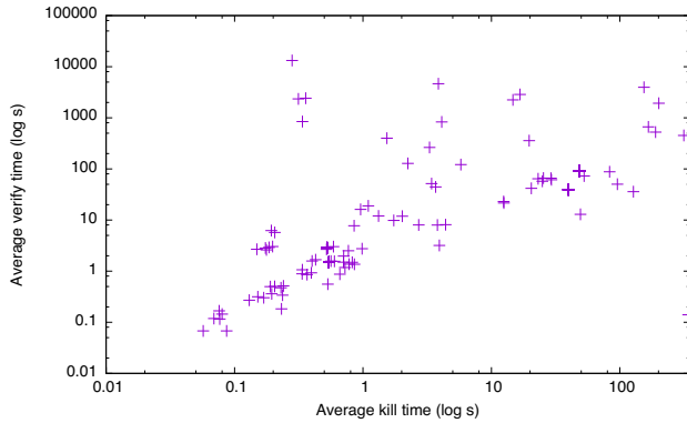
Fig. 13. Average times for killing/verifying mutants, in seconds.
